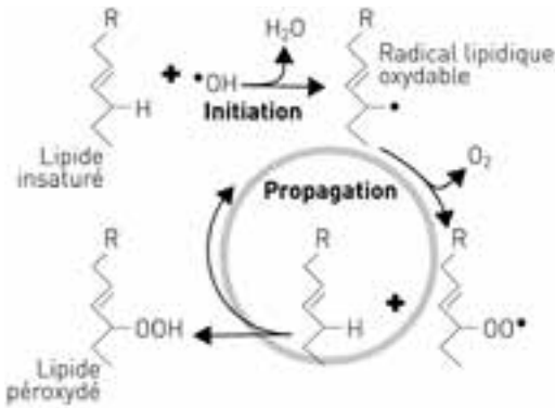
Figure 10 | Peroxydation.
