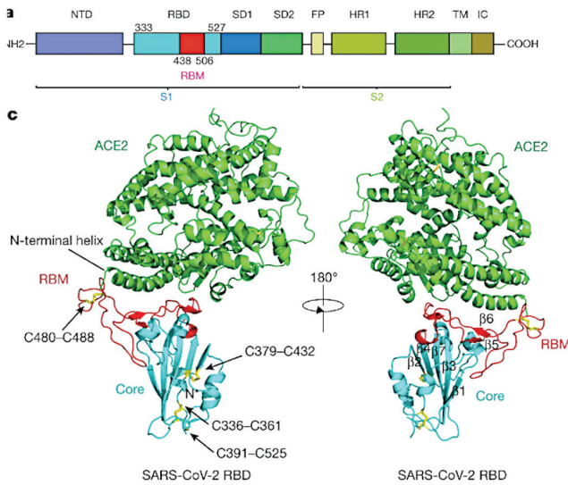
Structure of the SARS-CoV-2 spike receptor-binding domain bound to the ACE2 receptor Jun Lan et al., Nature, 2020 May;581(7807):215-220. doi: 10.1038/s41586-020-2180-5. Epub 2020 Mar 30.
