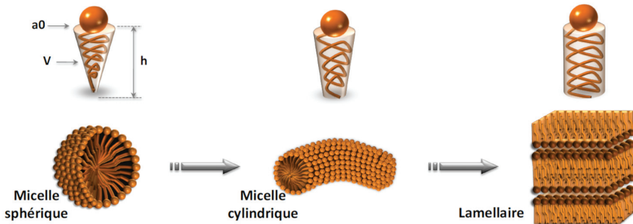
Figure 5. Micelles : formation et structures
